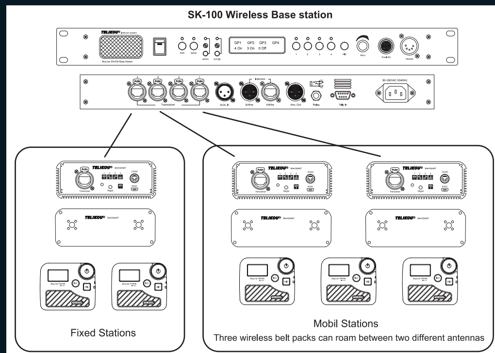
■ Application of SK-100 multi antennas
