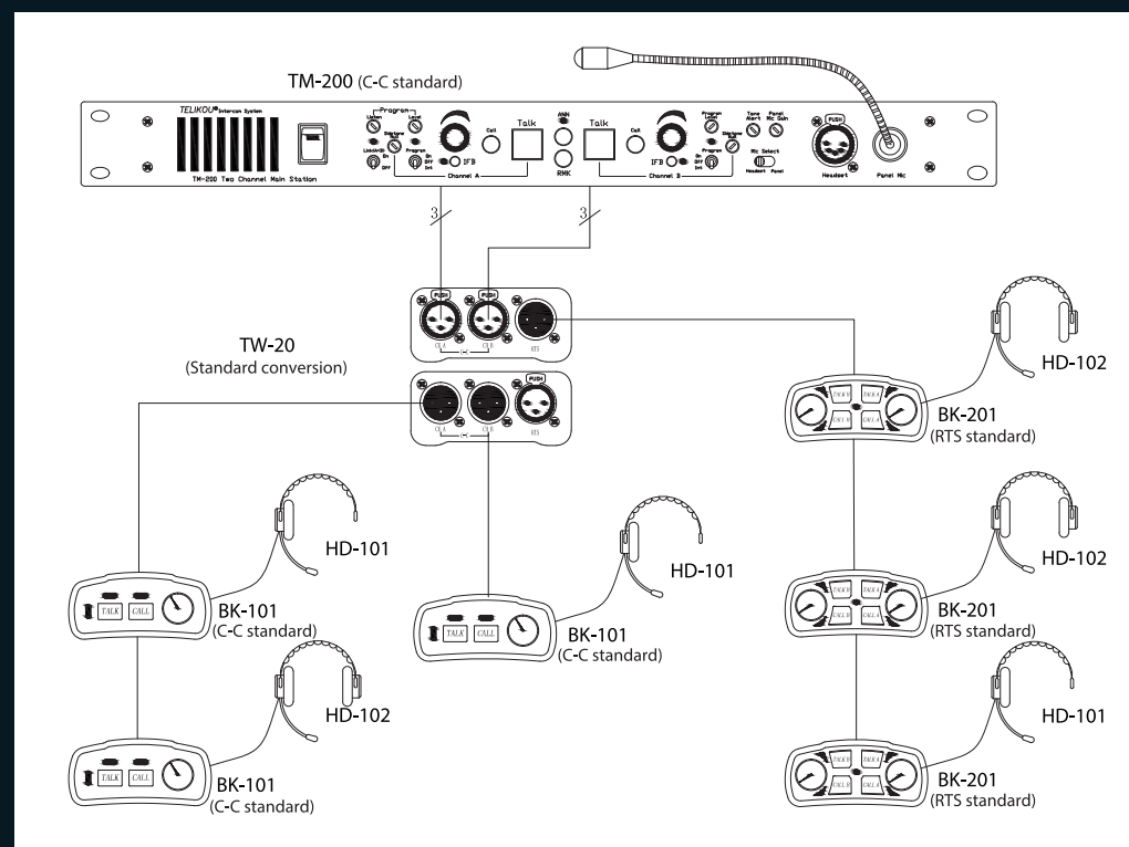
■ TW-20: The Conversion between Clear-Com and RTS Standard
